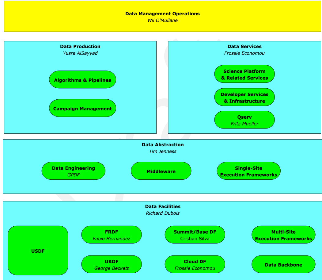
FIGURE 3: Functions in operations of Rubin Data Management.
